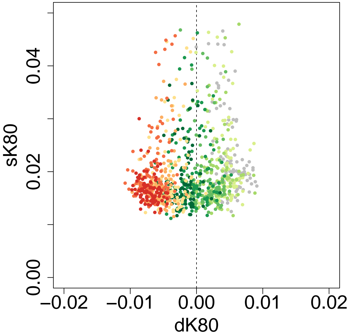
Scatter Plot: P3P2.OP2.tD12-0.1-tD13-0.4-tD14-3-tGF-0.05-len-25000 ghostflow: 0.2
