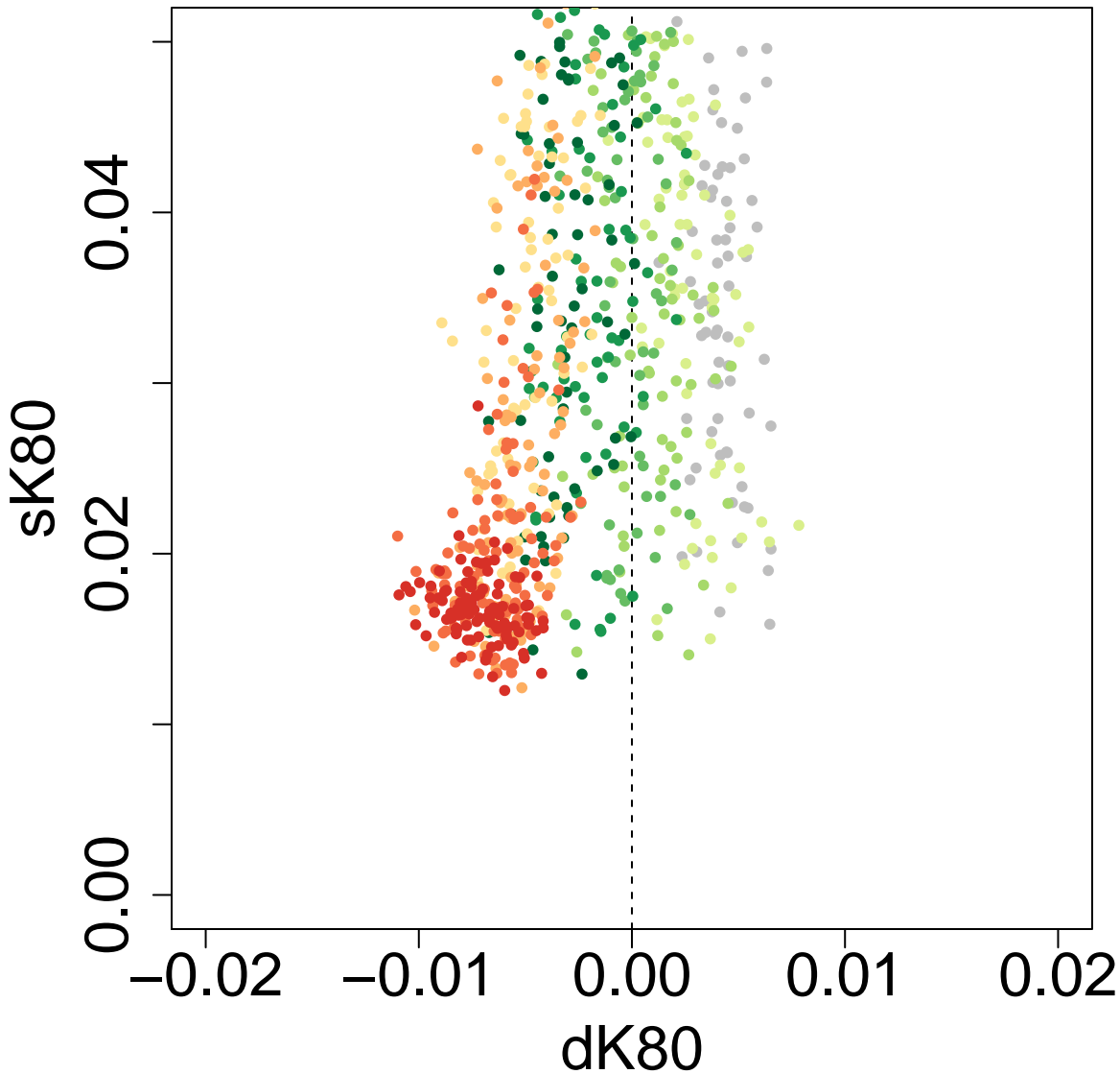
Scatter Plot: P3P2.OP2.tD12-0.1-tD13-0.4-tD14-3-tGF-0.05-len-25000 ghostflow: 0.4
