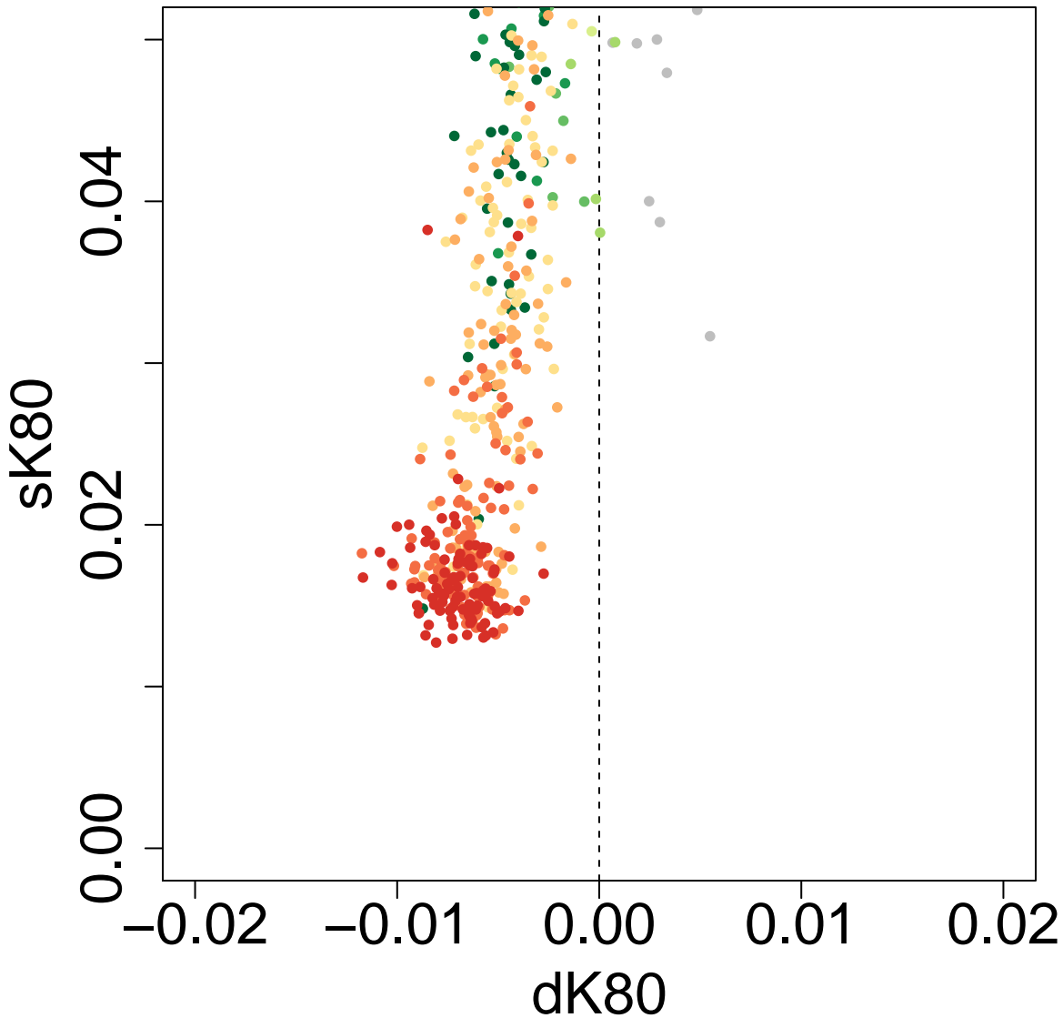
Scatter Plot: P3P2.OP2.tD12-0.1-tD13-0.4-tD14-3-tGF-0.05-len-25000 ghostflow: 0.6
