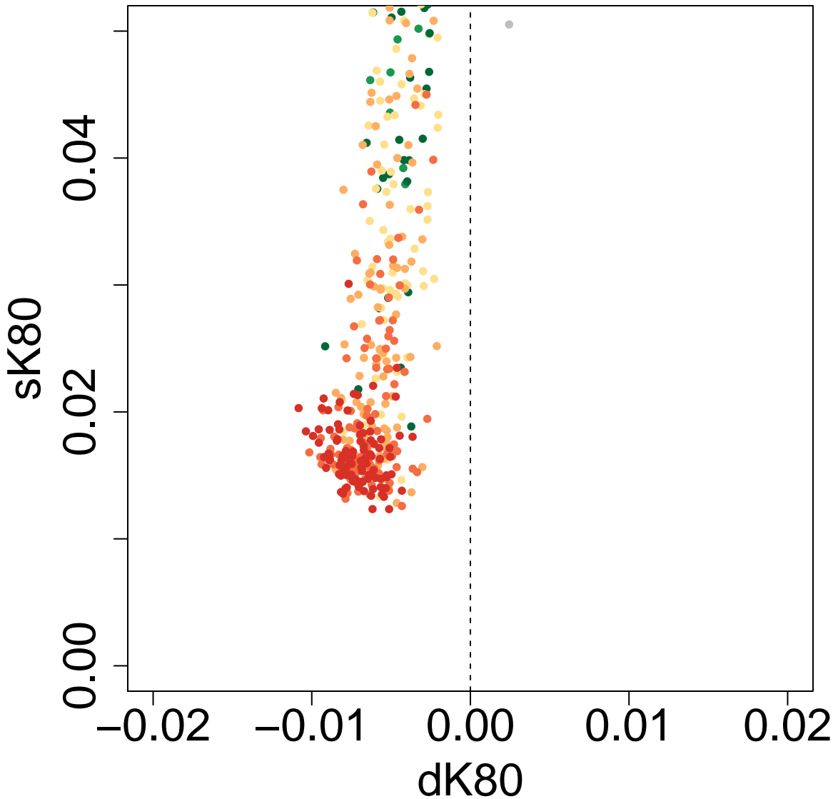
Scatter Plot: P3P2.OP2.tD12-0.1-tD13-0.4-tD14-3-tGF-0.05-len-25000 ghostflow: 0.7
