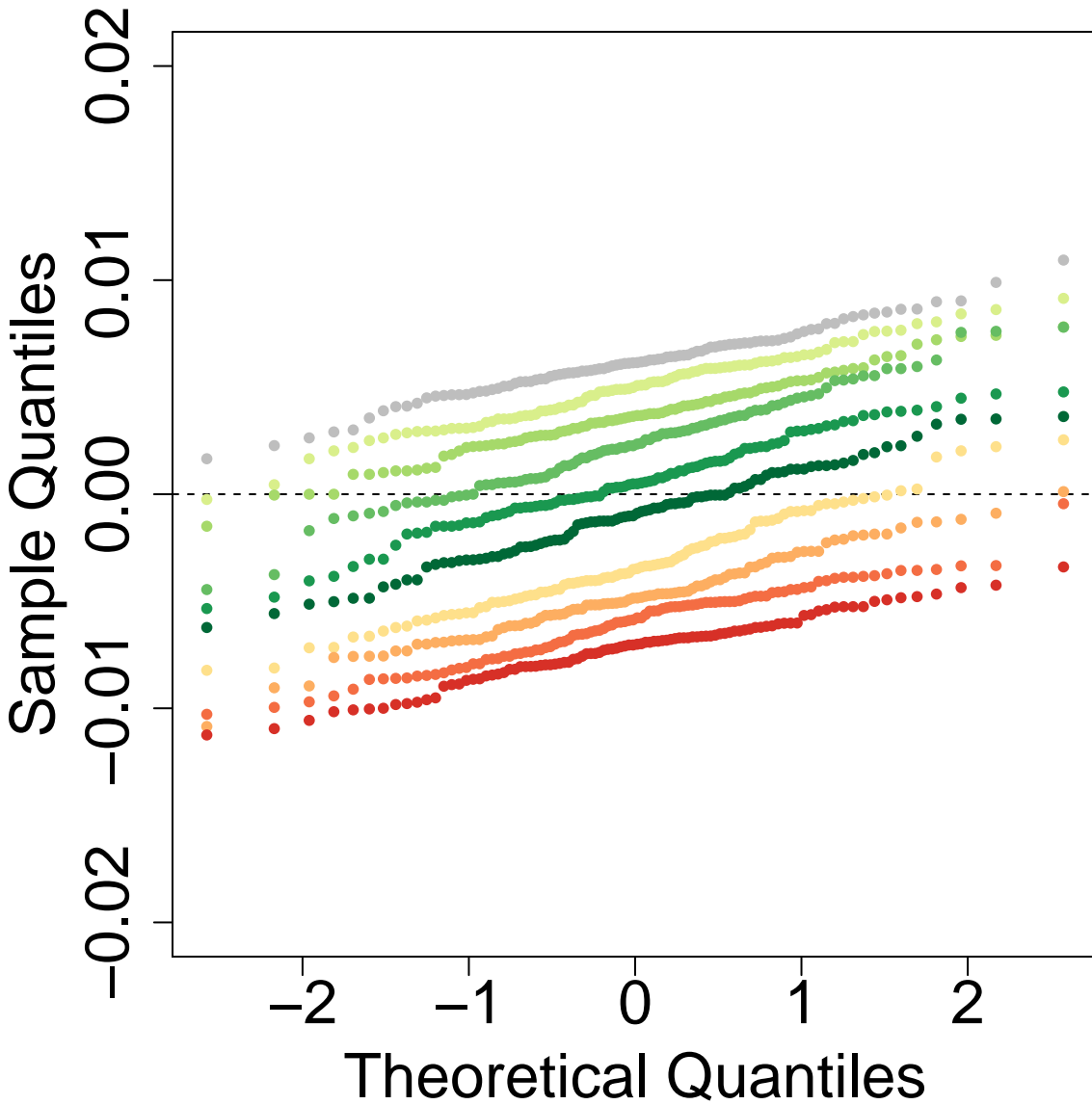
Q-Q Plot: P3P2.OP2.tD12-0.1-tD13-0.4-tD14-3-tGF-0.05-len-25000 ghostflow: 0.1
