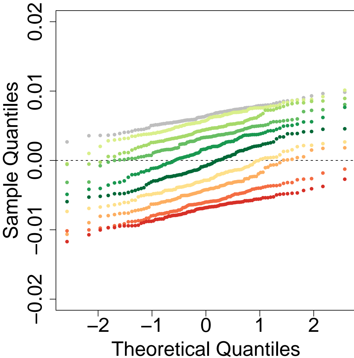
Q-Q Plot: P3P2.OP2.tD12-0.1-tD13-0.4-tD14-3-tGF-0.05-len-25000 ghostflow: 0
