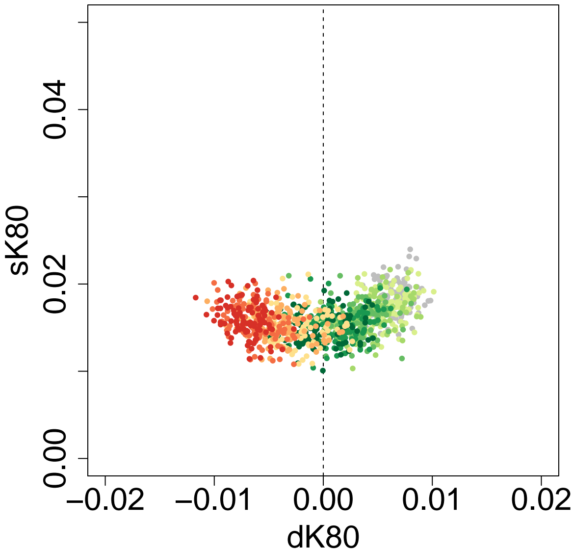
Scatter Plot: P3P2.OP2.tD12-0.1-tD13-0.4-tD14-3-tGF-0.05-len-25000 ghostflow: 0
