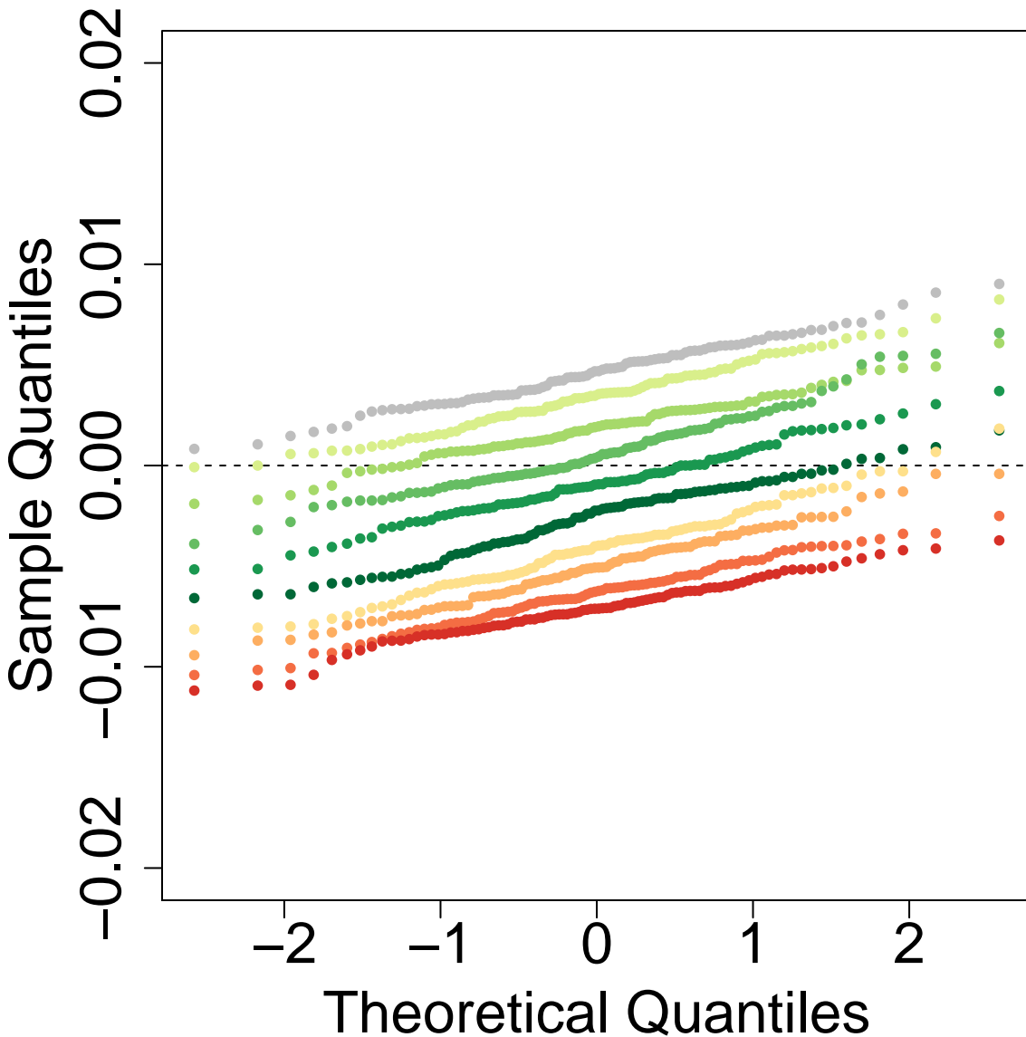
Q-Q Plot: P3P2.OP2.tD12-0.1-tD13-0.4-tD14-3-tGF-0.05-len-25000 ghostflow: 0.3
