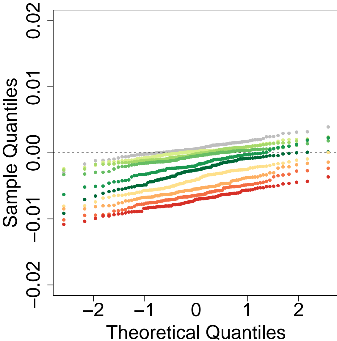
Q-Q Plot: P3P2.OP2.tD12-0.1-tD13-0.4-tD14-3-tGF-0.05-len-25000 ghostflow: 0.7
