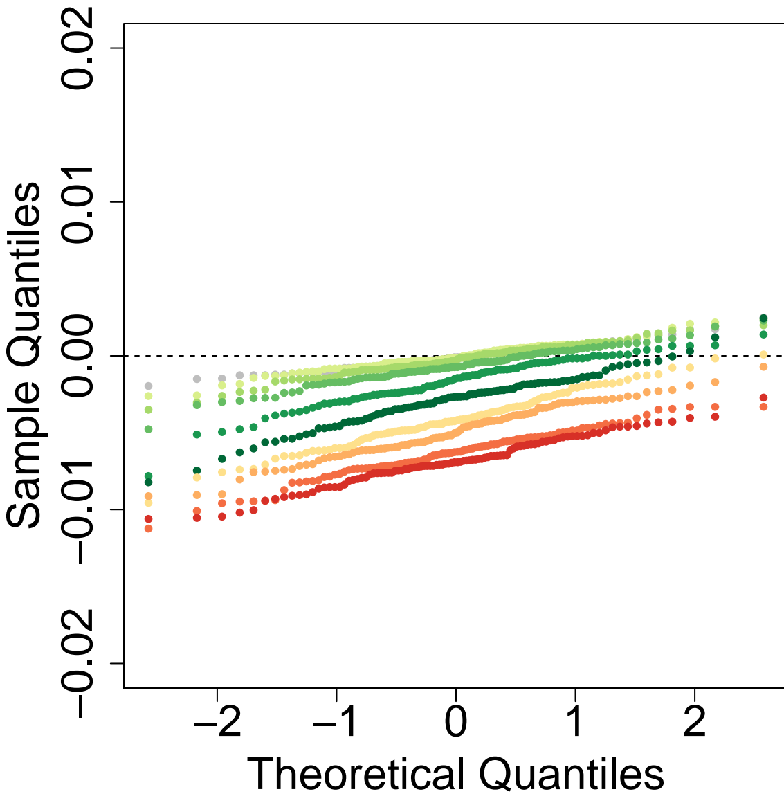
Q-Q Plot: P3P2.OP2.tD12-0.1-tD13-0.4-tD14-3-tGF-0.05-len-25000 ghostflow: 0.9
