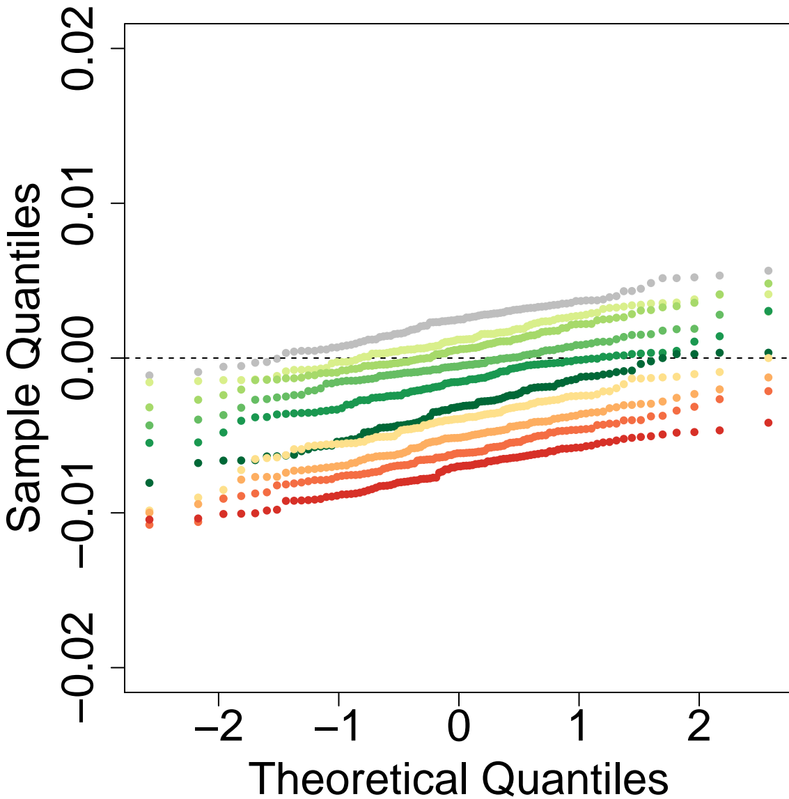
Q-Q Plot: P3P2.OP2.tD12-0.1-tD13-0.4-tD14-3-tGF-0.05-len-25000 ghostflow: 0.5
