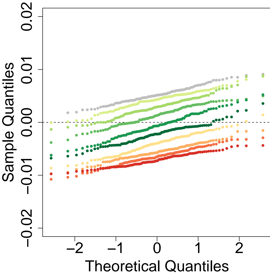
Q-Q Plot: P3P2.OP2.tD12-0.1-tD13-0.4-tD14-3-tGF-0.05-len-25000 ghostflow: 0.2
