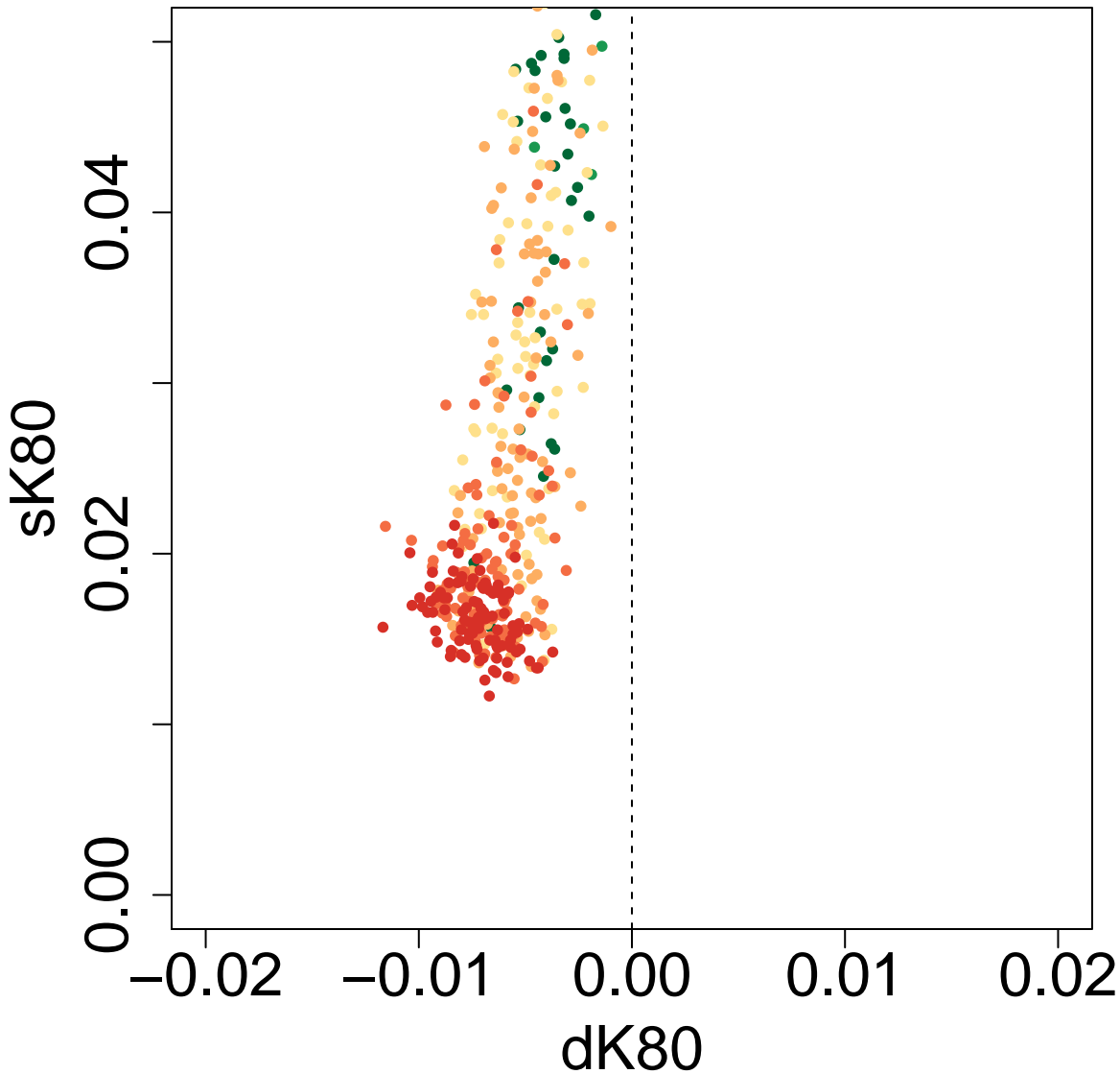
Scatter Plot: P3P2.OP2.tD12-0.1-tD13-0.4-tD14-3-tGF-0.05-len-25000 ghostflow: 1
