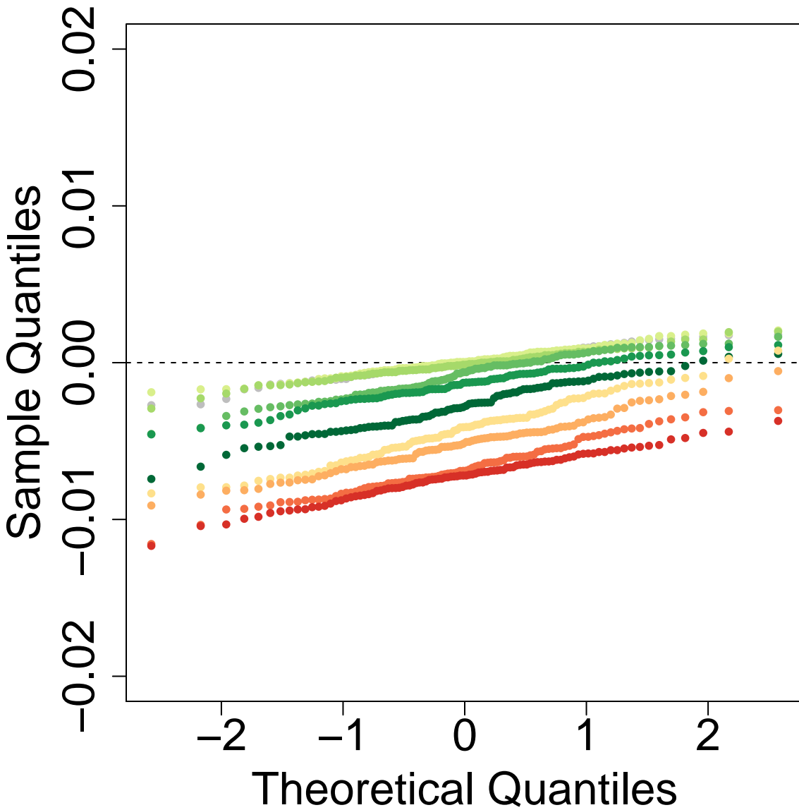
Q-Q Plot: P3P2.OP2.tD12-0.1-tD13-0.4-tD14-3-tGF-0.05-len-25000 ghostflow: 1
