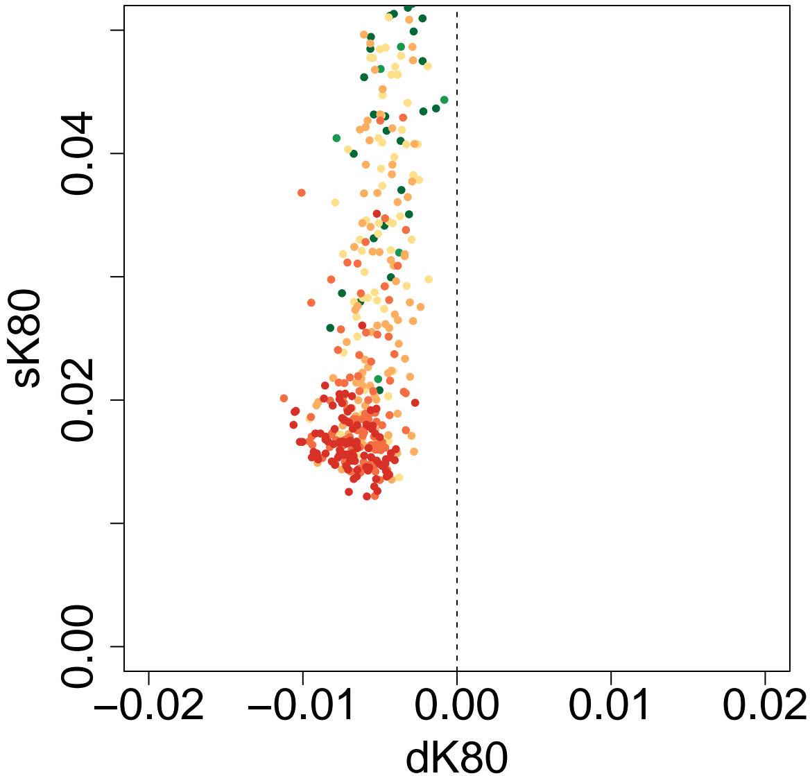
Scatter Plot: P3P2.OP2.tD12-0.1-tD13-0.4-tD14-3-tGF-0.05-len-25000 ghostflow: 0.9
