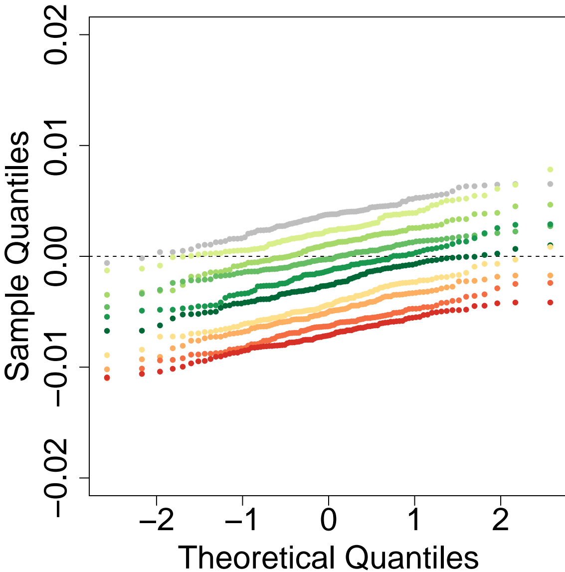
Q-Q Plot: P3P2.OP2.tD12-0.1-tD13-0.4-tD14-3-tGF-0.05-len-25000 ghostflow: 0.4
