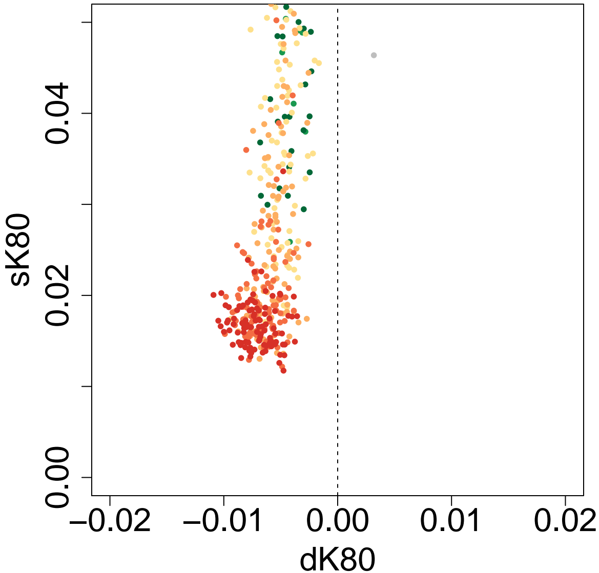
Scatter Plot: P3P2.OP2.tD12-0.1-tD13-0.4-tD14-3-tGF-0.05-len-25000 ghostflow: 0.8
