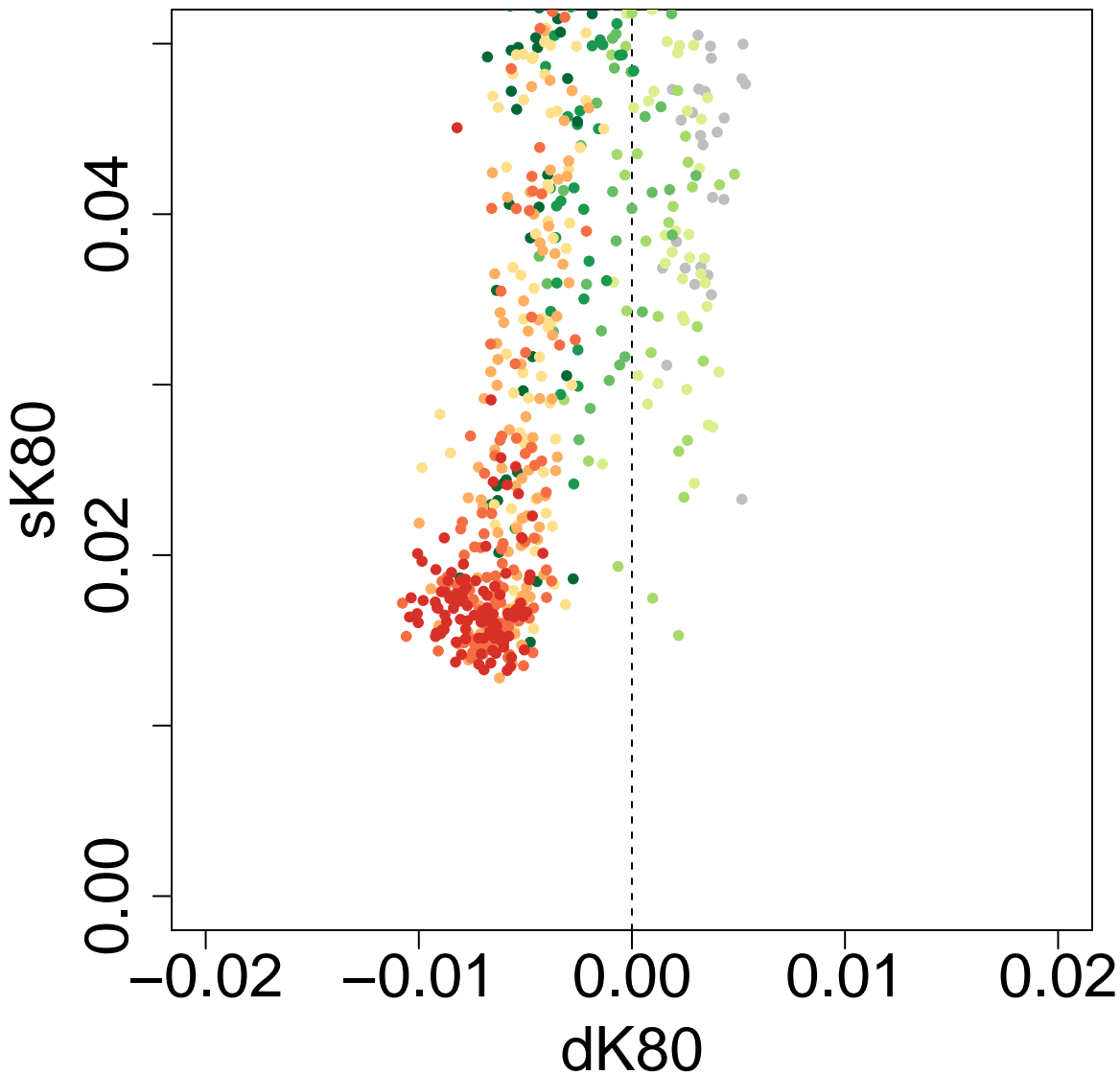
Scatter Plot: P3P2.OP2.tD12-0.1-tD13-0.4-tD14-3-tGF-0.05-len-25000 ghostflow: 0.5
