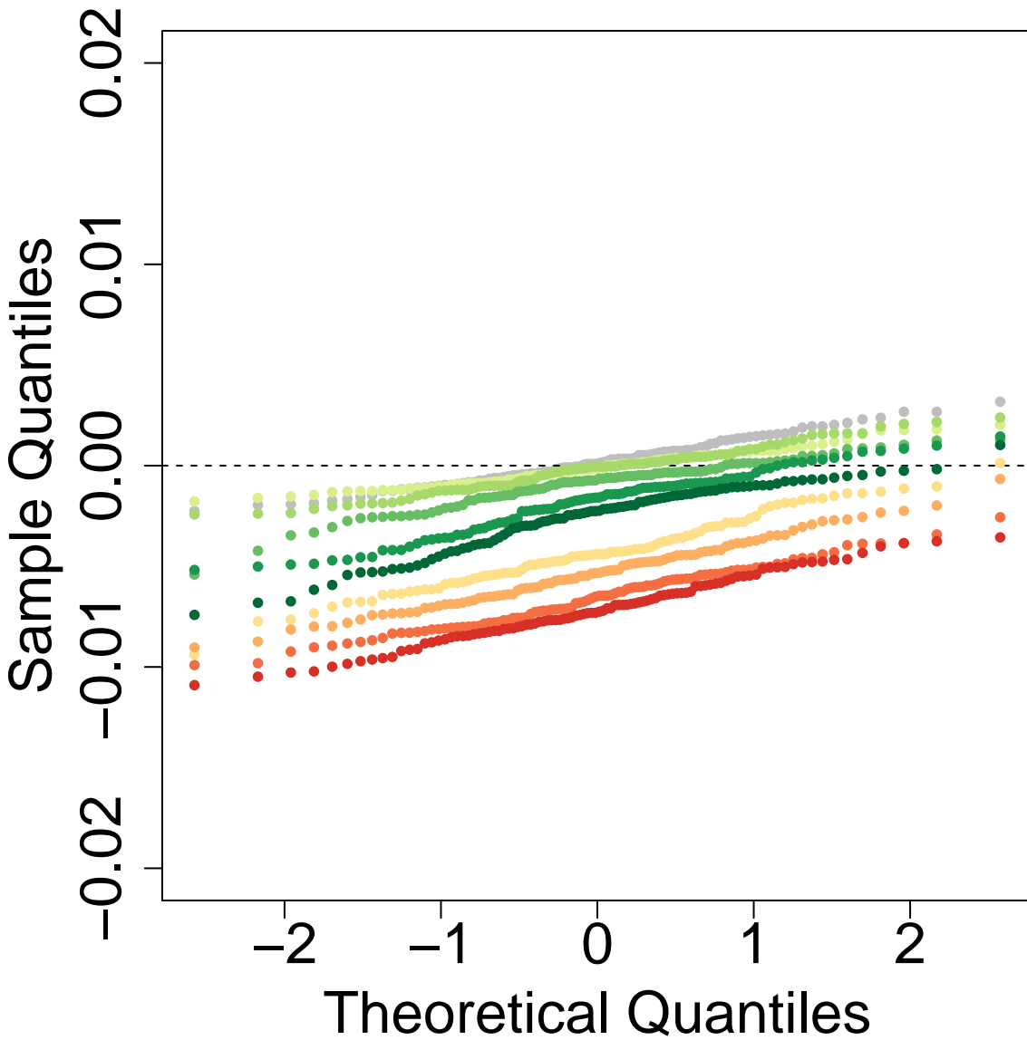
Q-Q Plot: P3P2.OP2.tD12-0.1-tD13-0.4-tD14-3-tGF-0.05-len-25000 ghostflow: 0.8
