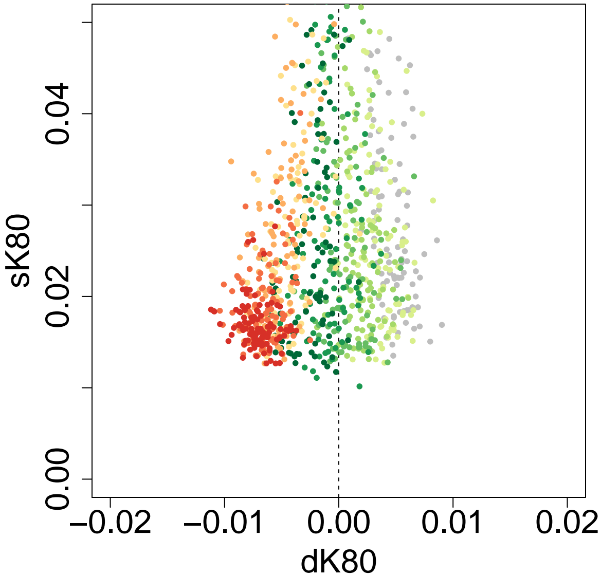
Scatter Plot: P3P2.OP2.tD12-0.1-tD13-0.4-tD14-3-tGF-0.05-len-25000 ghostflow: 0.3
