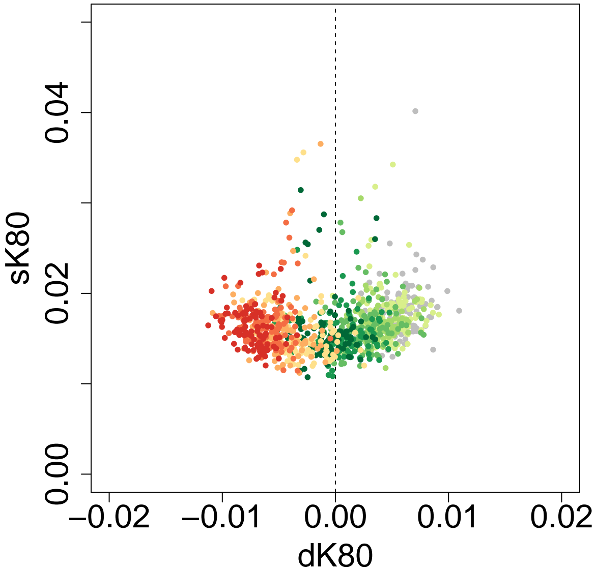
Scatter Plot: P3P2.OP2.tD12-0.1-tD13-0.4-tD14-3-tGF-0.05-len-25000 ghostflow: 0.1
