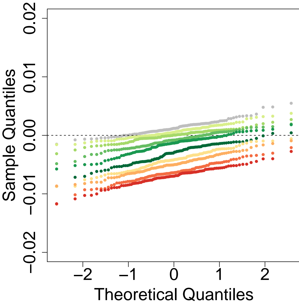
Q-Q Plot: P3P2.OP2.tD12-0.1-tD13-0.4-tD14-3-tGF-0.05-len-25000 ghostflow: 0.6
