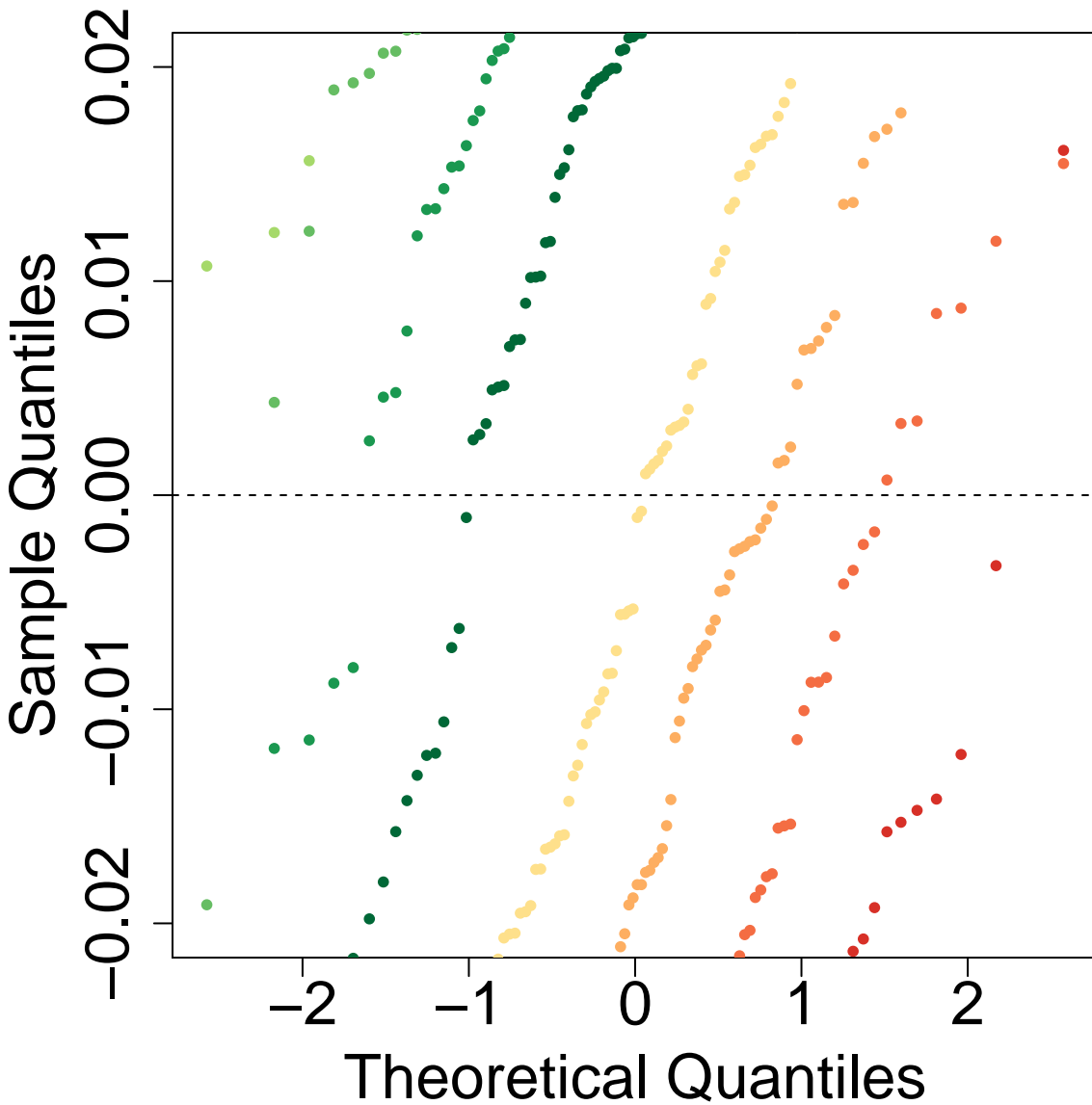
Q-Q Plot: P3P2.OP3.tD12-0.1-tD13-0.4-tD14-3-tGF-0.05-len-25000 ghostflow: 0.8
