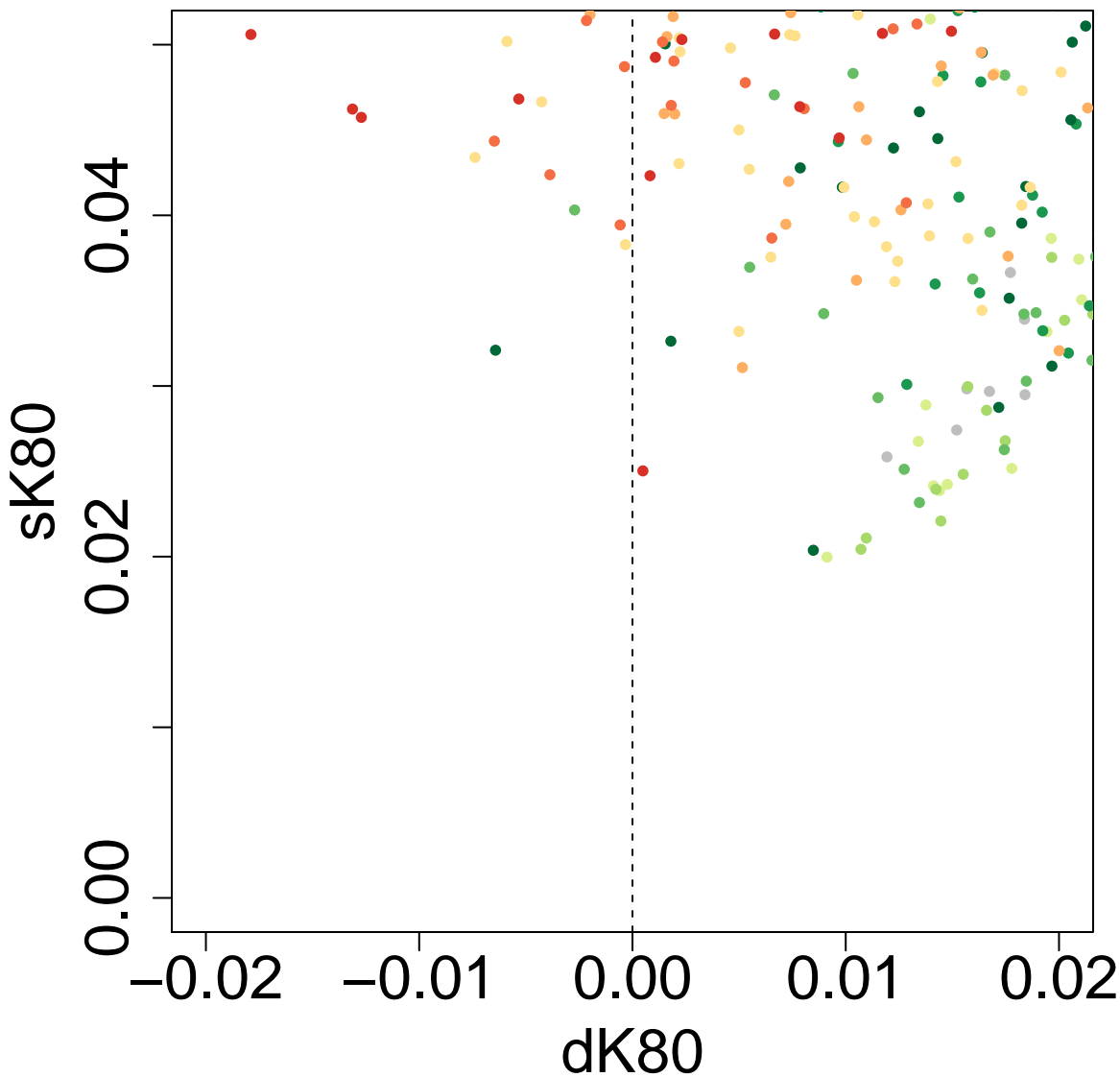
Scatter Plot: P3P2.OP3.tD12-0.1-tD13-0.4-tD14-3-tGF-0.05-len-25000 ghostflow: 0.6
