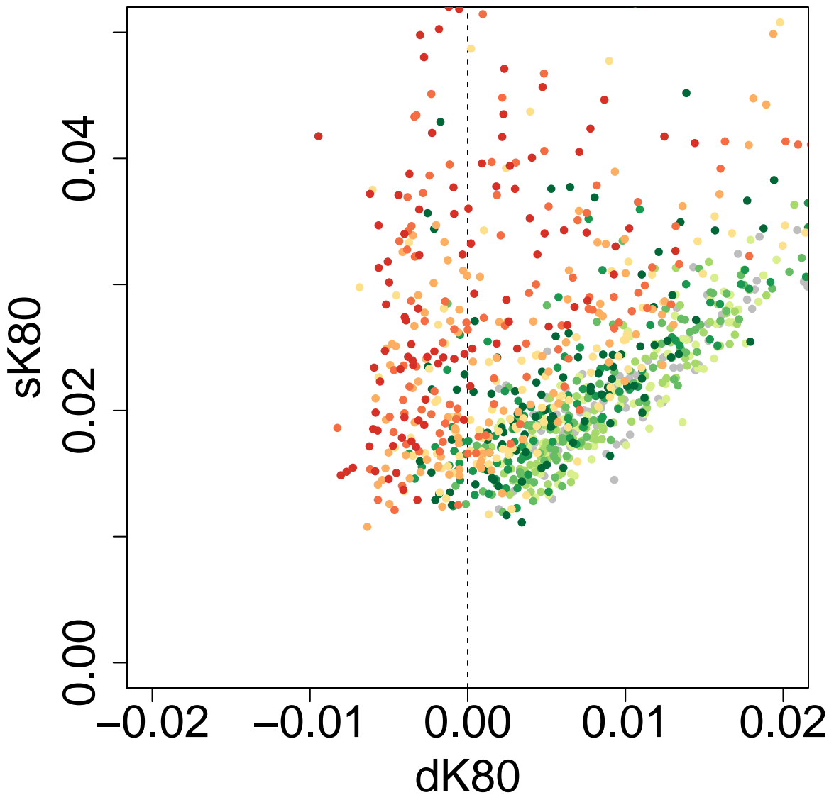
Scatter Plot: P3P2.OP3.tD12-0.1-tD13-0.4-tD14-3-tGF-0.05-len-25000 ghostflow: 0.3
