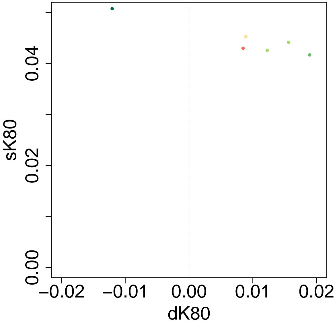
Scatter Plot: P3P2.OP3.tD12-0.1-tD13-0.4-tD14-3-tGF-0.05-len-25000 ghostflow: 0.8
