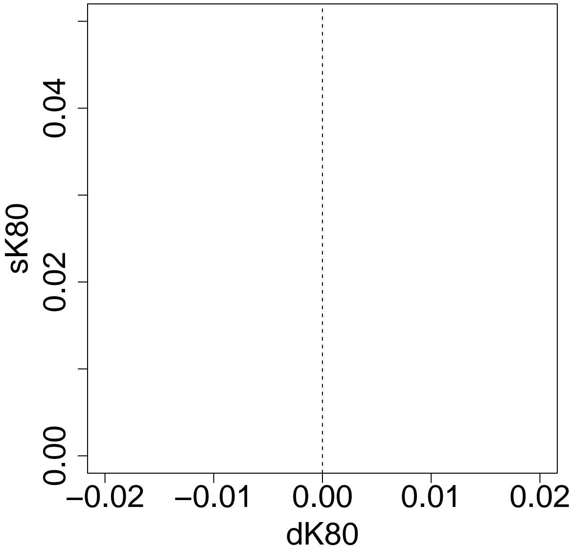
Scatter Plot: P3P2.OP3.tD12-0.1-tD13-0.4-tD14-3-tGF-0.05-len-25000 ghostflow: 0.9
