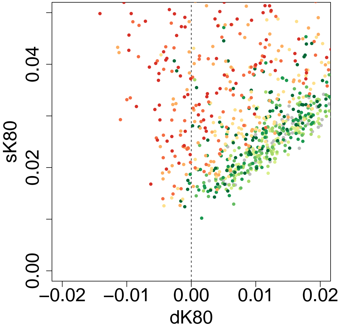
Scatter Plot: P3P2.OP3.tD12-0.1-tD13-0.4-tD14-3-tGF-0.05-len-25000 ghostflow: 0.4
