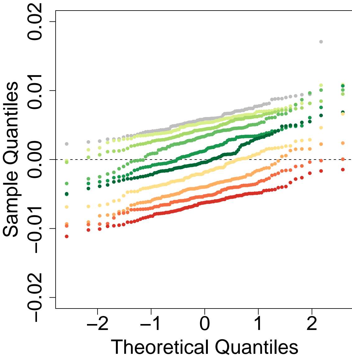
Q-Q Plot: P3P2.OP3.tD12-0.1-tD13-0.4-tD14-3-tGF-0.05-len-25000 ghostflow: 0.1
