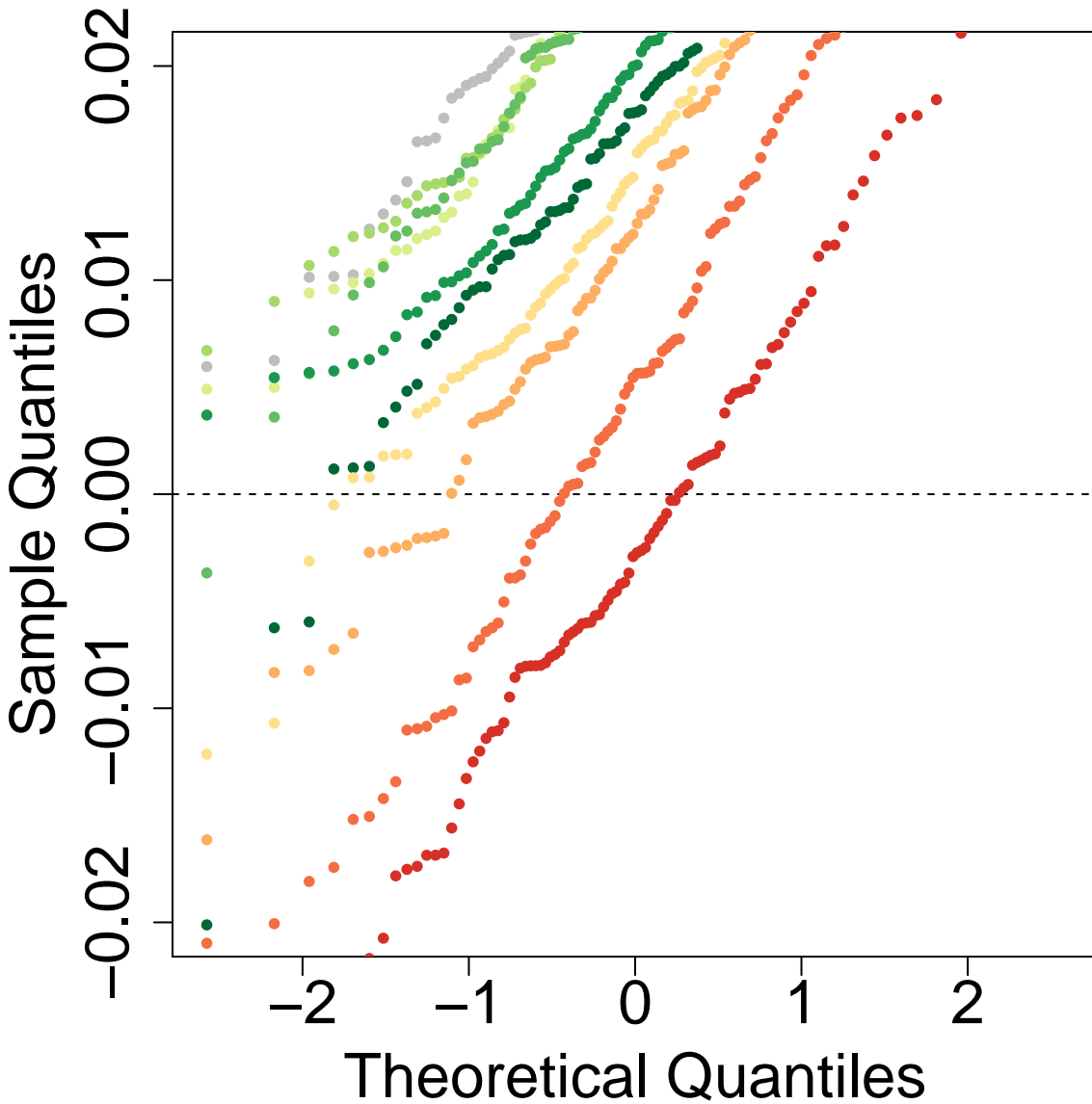
Q-Q Plot: P3P2.OP3.tD12-0.1-tD13-0.4-tD14-3-tGF-0.05-len-25000 ghostflow: 0.5
