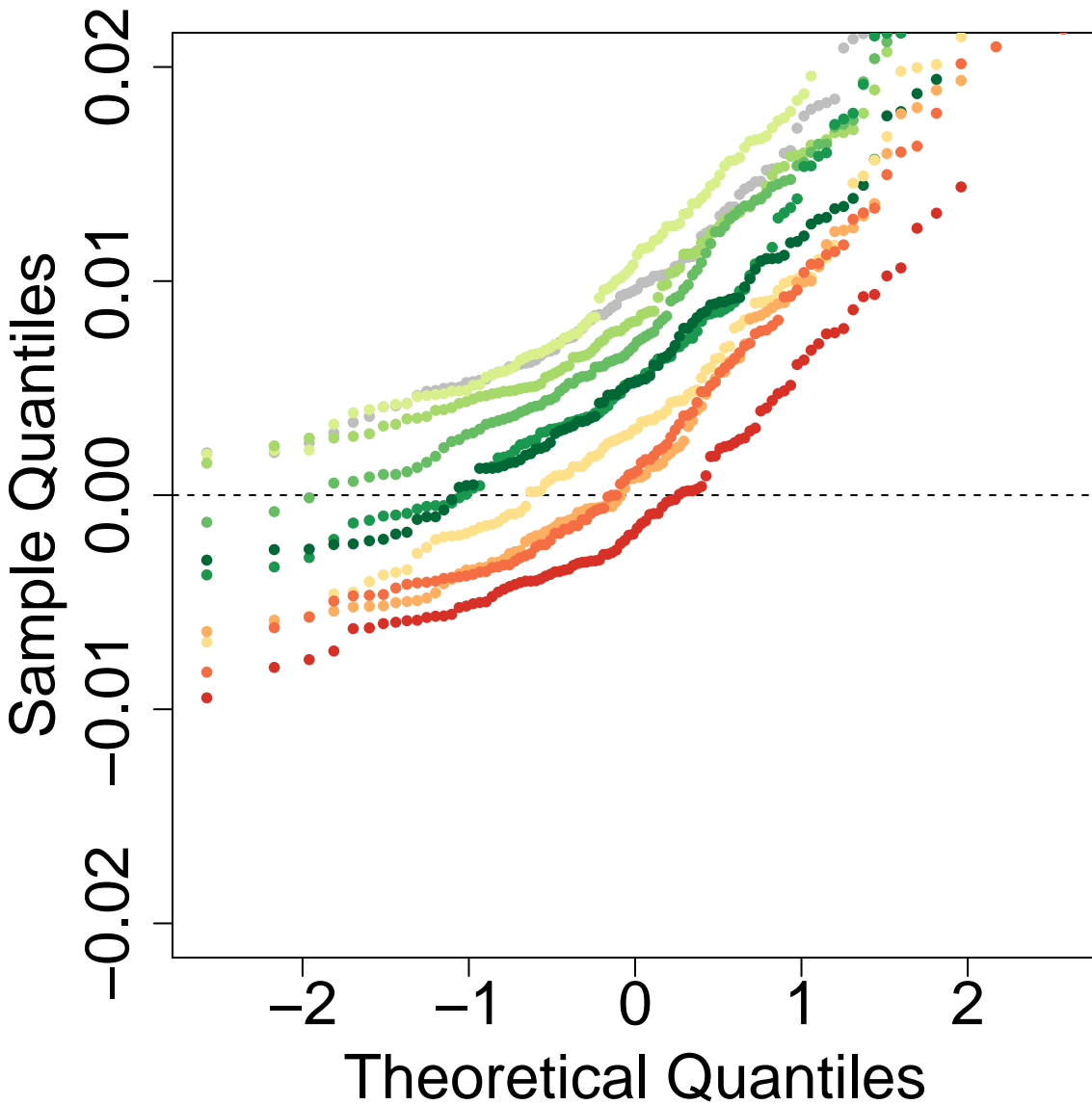
Q-Q Plot: P3P2.OP3.tD12-0.1-tD13-0.4-tD14-3-tGF-0.05-len-25000 ghostflow: 0.3
