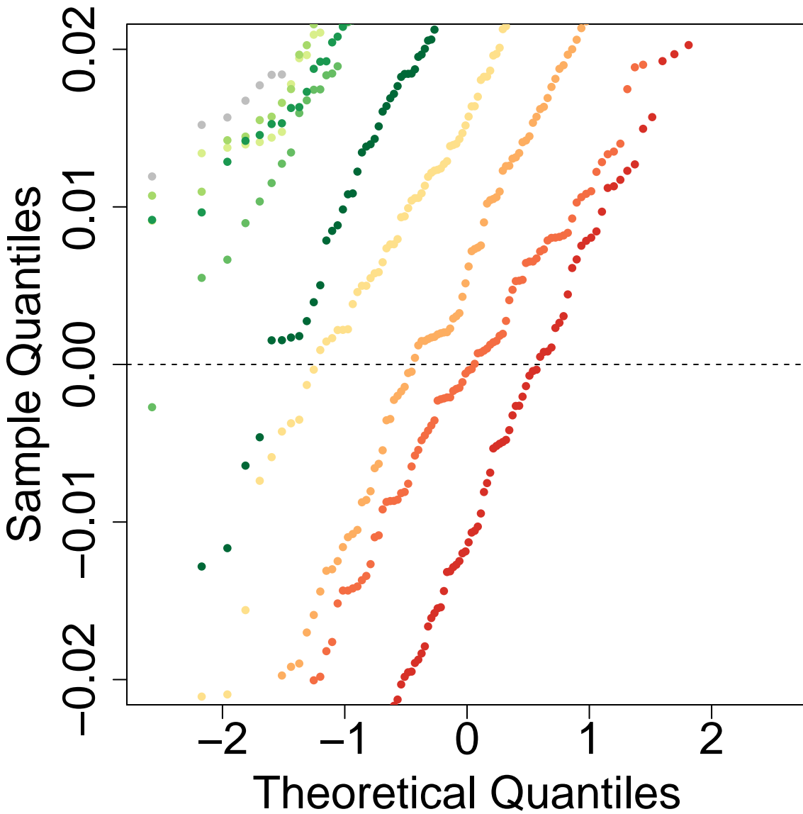
Q-Q Plot: P3P2.OP3.tD12-0.1-tD13-0.4-tD14-3-tGF-0.05-len-25000 ghostflow: 0.6
