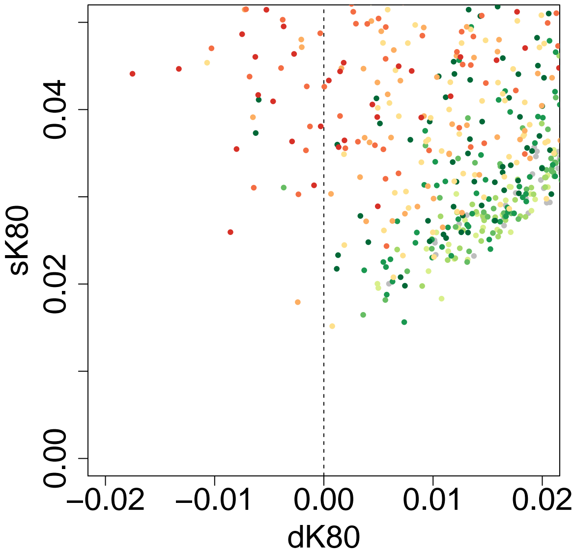
Scatter Plot: P3P2.OP3.tD12-0.1-tD13-0.4-tD14-3-tGF-0.05-len-25000 ghostflow: 0.5
