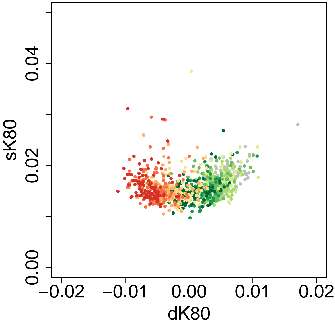
Scatter Plot: P3P2.OP3.tD12-0.1-tD13-0.4-tD14-3-tGF-0.05-len-25000 ghostflow: 0.1
