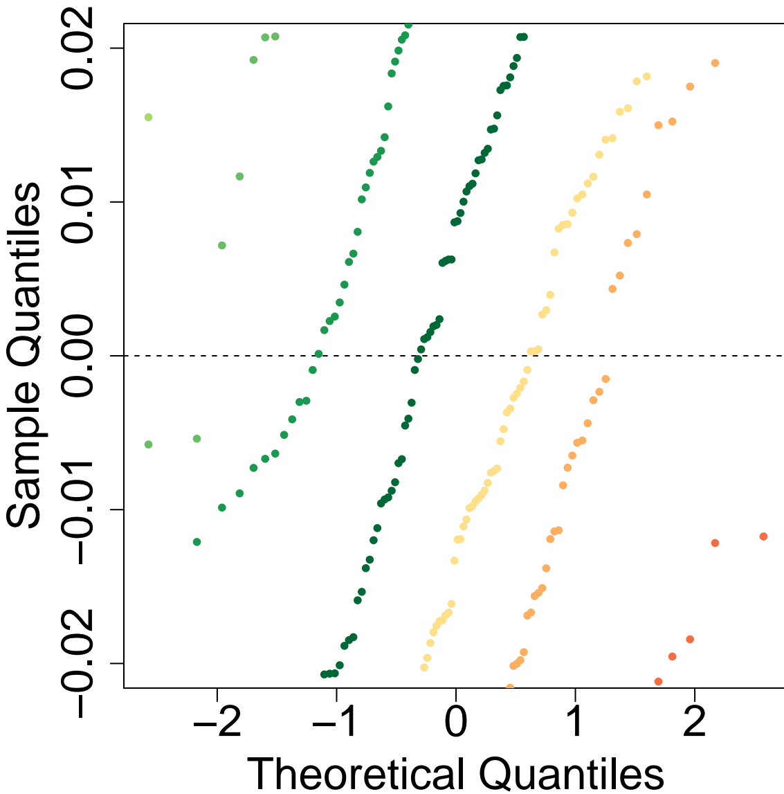
Q-Q Plot: P3P2.OP3.tD12-0.1-tD13-0.4-tD14-3-tGF-0.05-len-25000 ghostflow: 0.9
