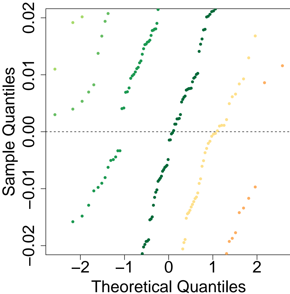
Q-Q Plot: P3P2.OP3.tD12-0.1-tD13-0.4-tD14-3-tGF-0.05-len-25000 ghostflow: 1
