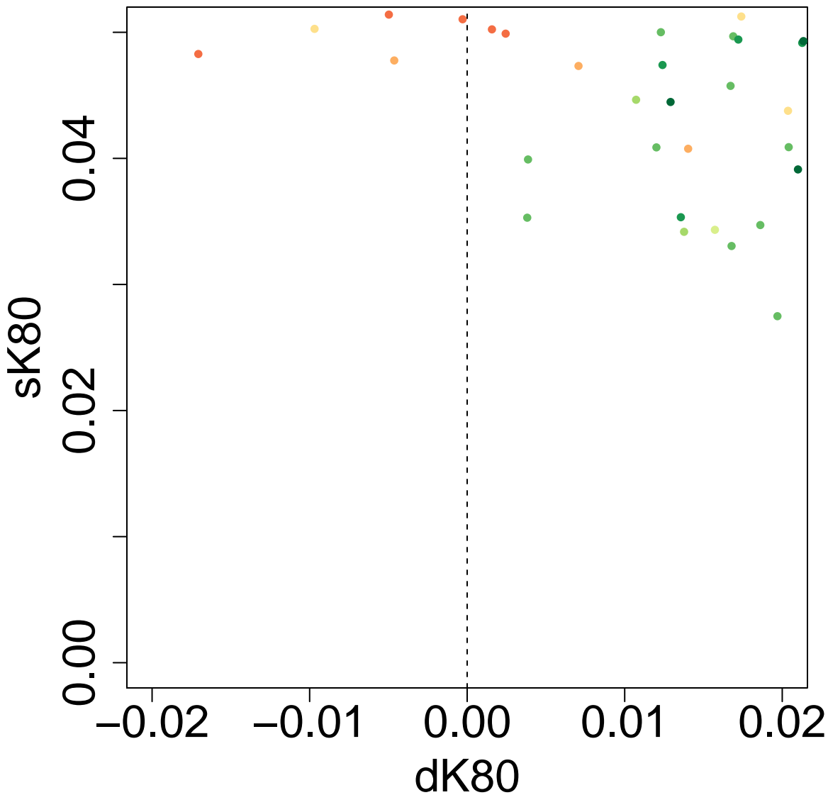
Scatter Plot: P3P2.OP3.tD12-0.1-tD13-0.4-tD14-3-tGF-0.05-len-25000 ghostflow: 0.7
