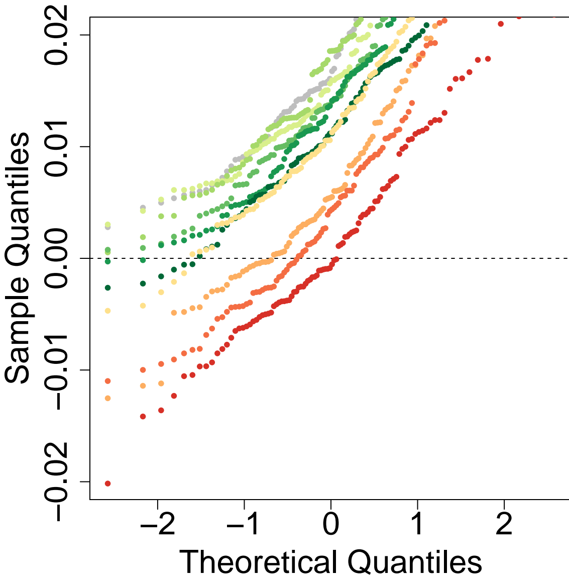
Q-Q Plot: P3P2.OP3.tD12-0.1-tD13-0.4-tD14-3-tGF-0.05-len-25000 ghostflow: 0.4
