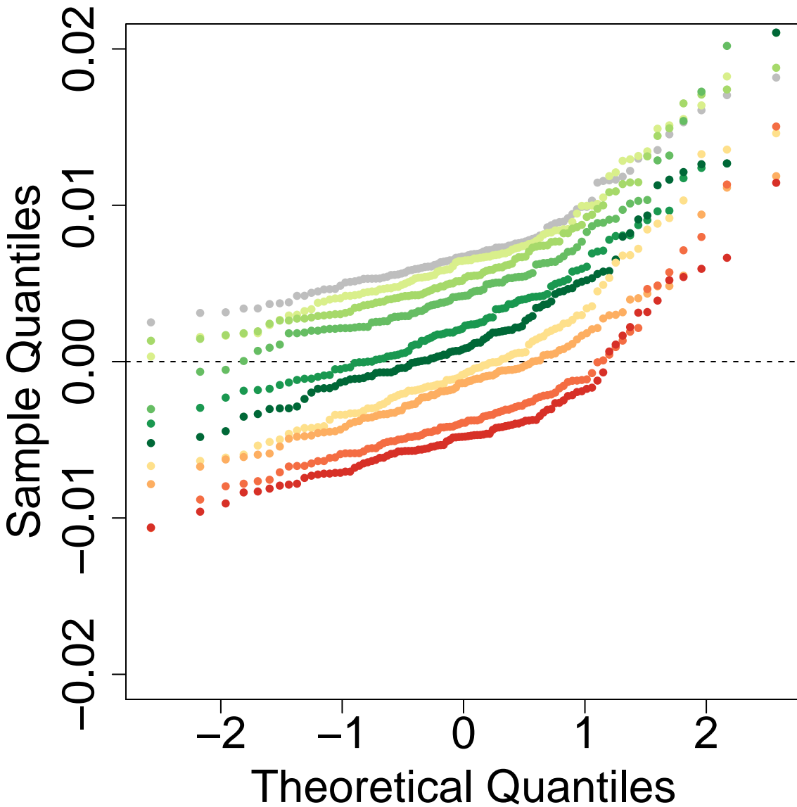
Q-Q Plot: P3P2.OP3.tD12-0.1-tD13-0.4-tD14-3-tGF-0.05-len-25000 ghostflow: 0.2
