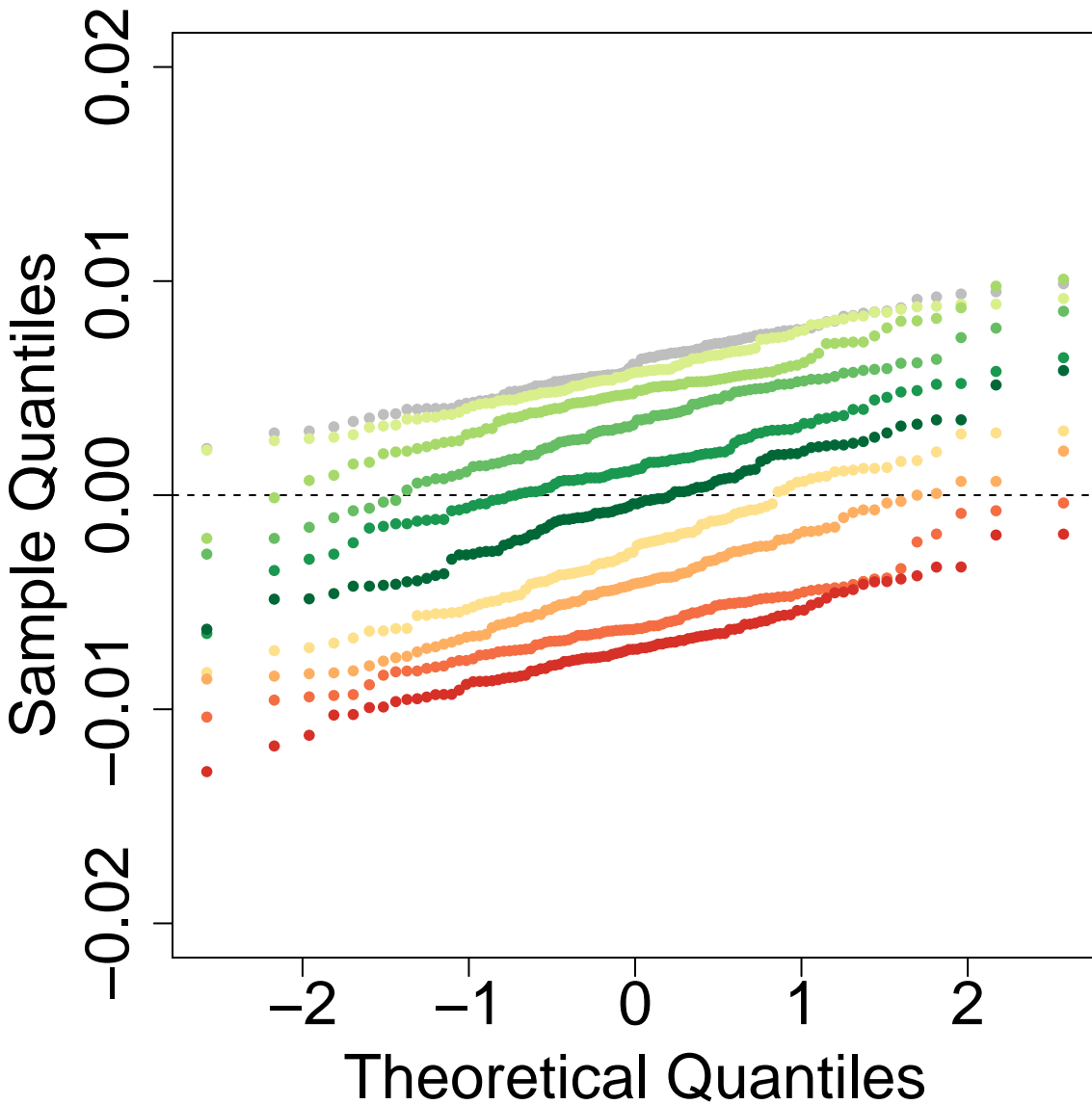
Q-Q Plot: P3P2.OP3.tD12-0.1-tD13-0.4-tD14-3-tGF-0.05-len-25000 ghostflow: 0
