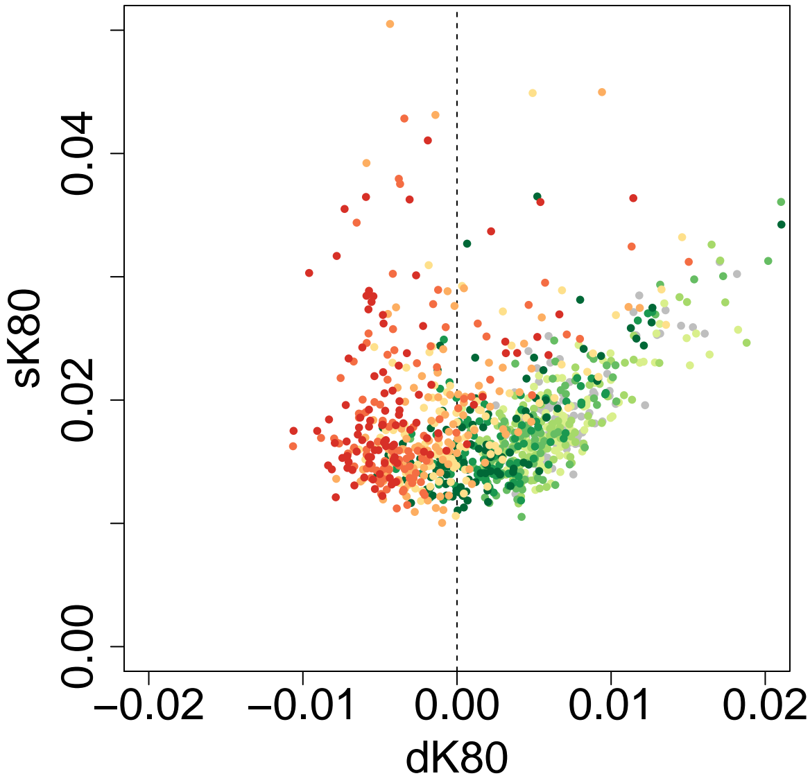
Scatter Plot: P3P2.OP3.tD12-0.1-tD13-0.4-tD14-3-tGF-0.05-len-25000 ghostflow: 0.2
