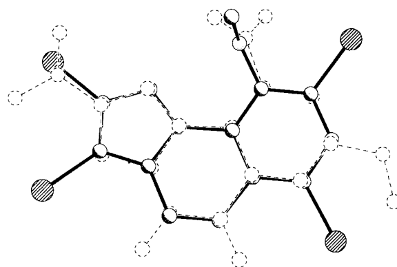
Fig. 1. Molecular Conformations of the Tetrabromopseudilin 9a (Bold Lines), Methoxatin ( 10a , Dotted Lines)
