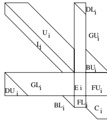
Figure 14: Factored local matrix
