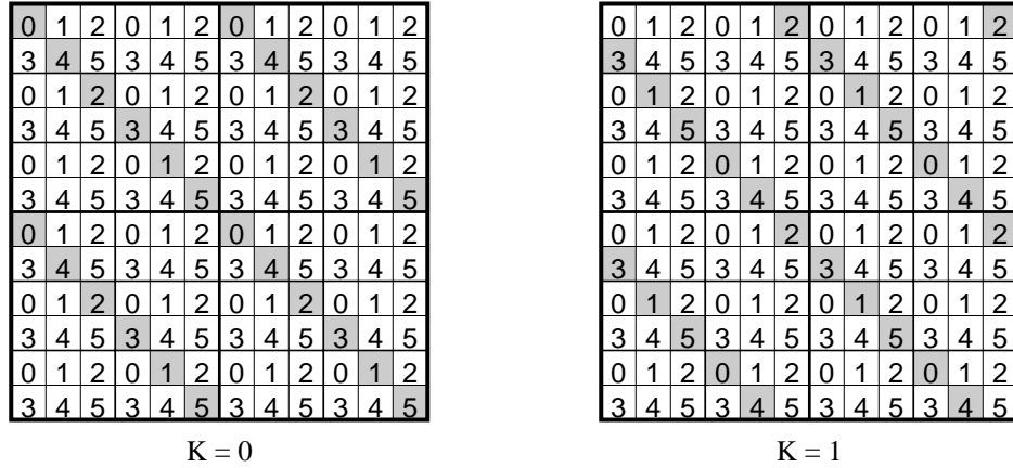
Figure 6: Snapshot of MB algorithm. In this case P = 2 , Q = 3 , and so the LCM of P and Q is 6. In each stage, two (\lfloor L \quad b / LCM \rfloor = 12 / 6) wrapped diagonals are broadcast. The total number of stages is LCM.
