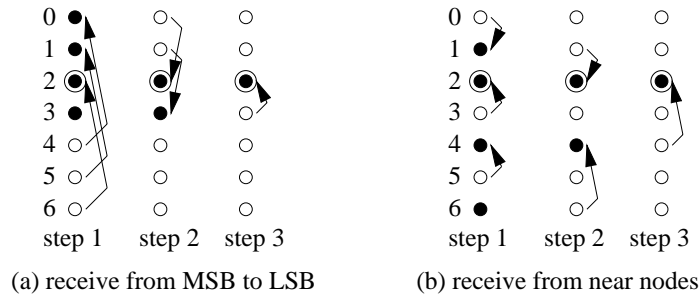
Figure 23: Collecting on linear array. P is a root node.
