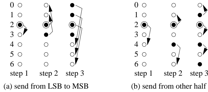
Figure 22: Broadcasting on linear array of p = 7 , where nodes are numbered 0 through 6. P is a root node.
