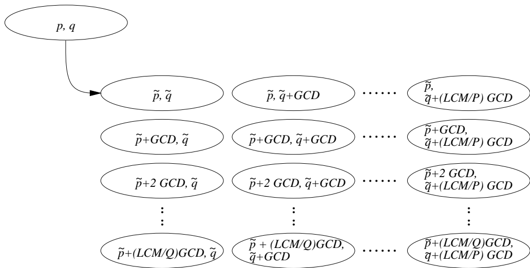
Figure 10: Processor map for communication. A processor P\langle p, q \rangle starts to communicate with P\langle \tilde{p}, \tilde{q} \rangle , then it communicates with other processors, whose vertical and horizontal intervals are GCD from P\langle \tilde{p}, \tilde{q} \rangle .
