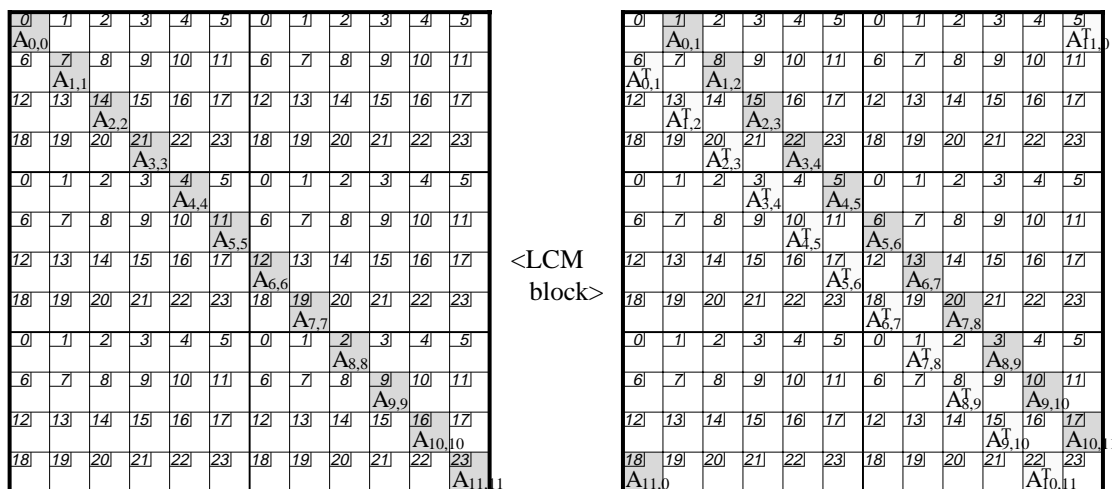
Figure 11: A modified matrix transpose algorithm from the processor point-of-view. Operations of GCD groups of processors are overlapped.
