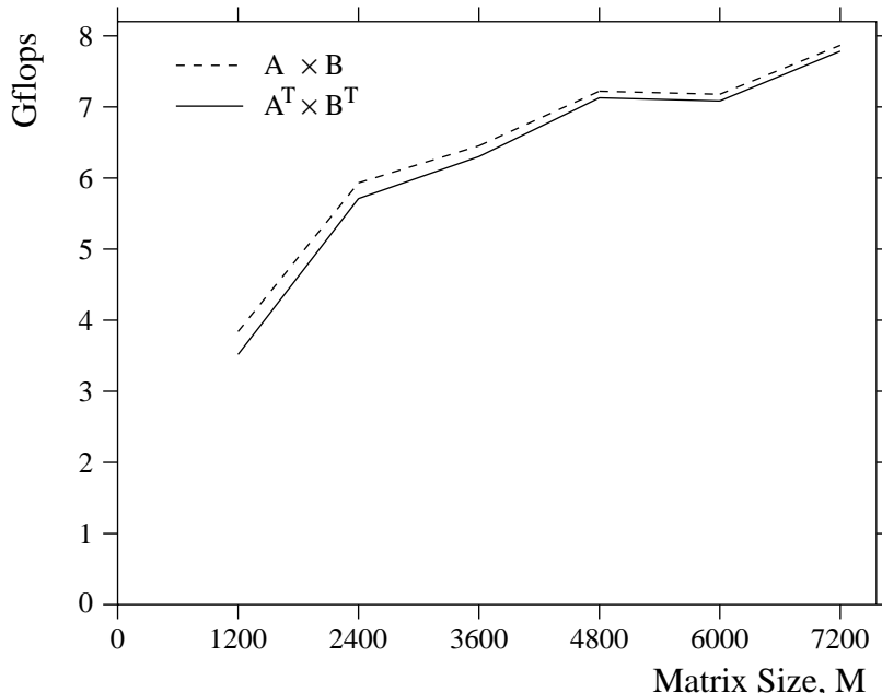
Figure 15: Performance comparison of \mathbf{A} \cdot \mathbf{B} and \mathbf{A}^T \cdot \mathbf{B}^T on 15 \times 16 template. ( P = 15, Q = 16 , and GCD = 1 ). \mathbf{C} \leftarrow \mathbf{A}^T \cdot \mathbf{B}^T is implemented in two steps, \mathbf{T} \leftarrow \mathbf{B} \cdot \mathbf{A} , and then \mathbf{C} \leftarrow \mathbf{T}^T .
